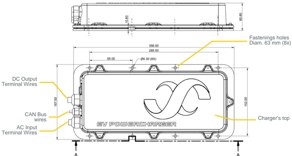
Figure 2 Mounting screws and dimensions for the EV Power Chargers 3kW HE, IP67
